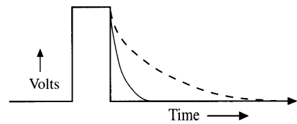
Fig. 4. Polarprobe electrical relaxation curves. Two curves are depicted, each showing different electrical decay constants.
