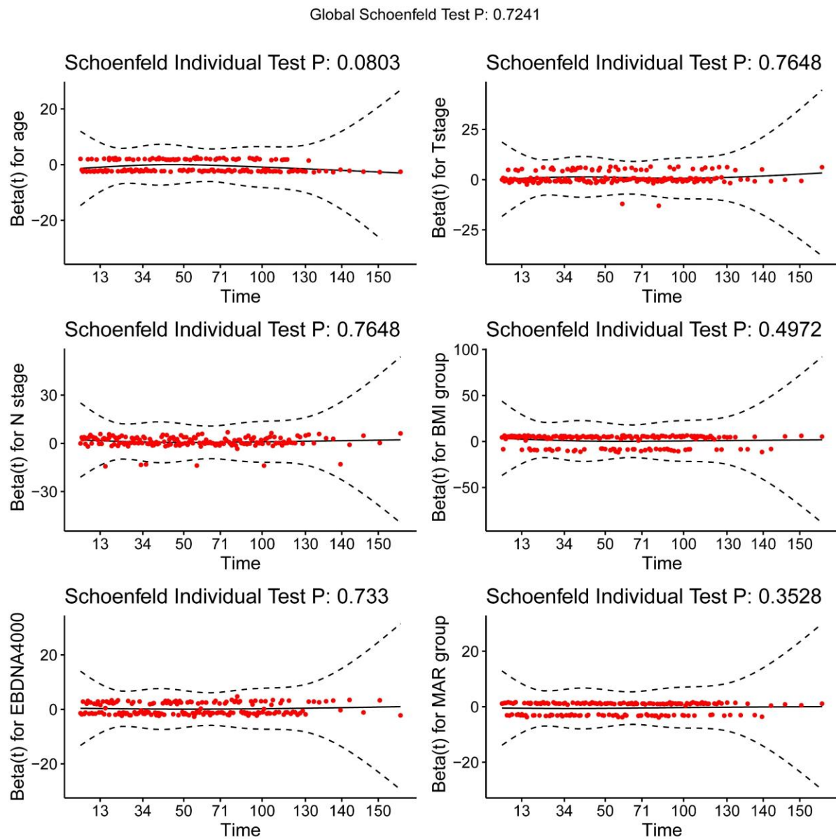
Fig. S2. Proportional hazards diagnostic plot.
